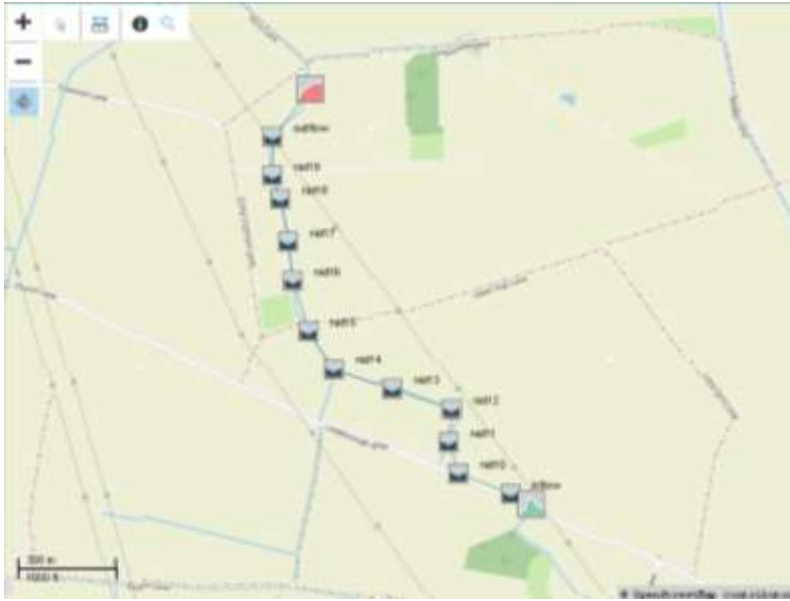
Figure 4.4: New Ings Drain (North) 1D Node Location
