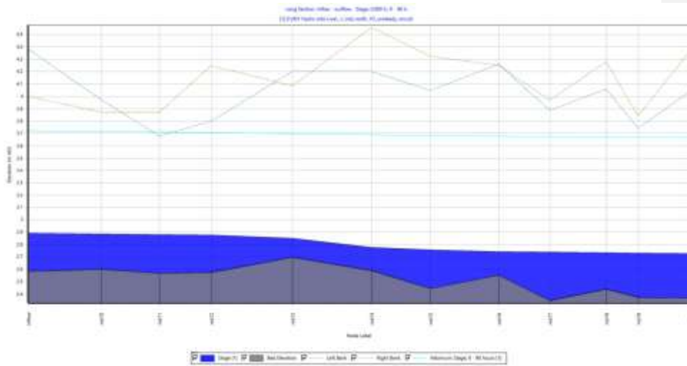
Figure 4.16203.7: New Ings Drain (North) in 100 year + 23% Unsteady Simulation Long Section
